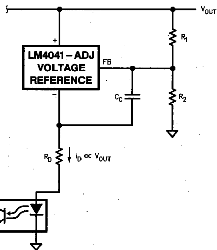
FIGURE 17. Opto-Coupler Feedback Circuit
