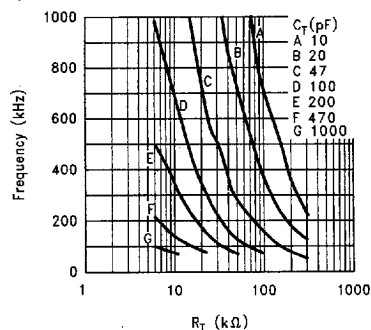
FIGURE 1. Frequency vs R_T and C_T Graph
