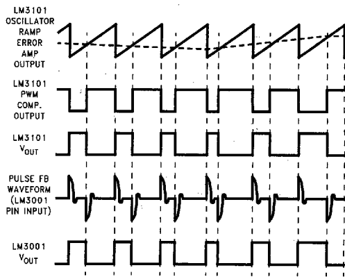
FIGURE 14. Pulse Feedback Timing Diagram
