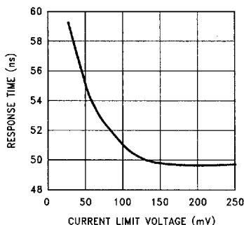
FIGURE 16. Current Limit Response Time
