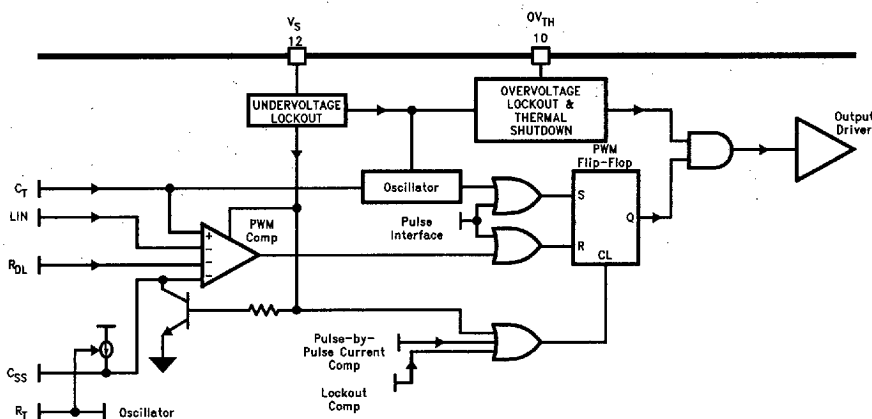
FIGURE 8. Overvoltage/Undervoltage Block Diagram
