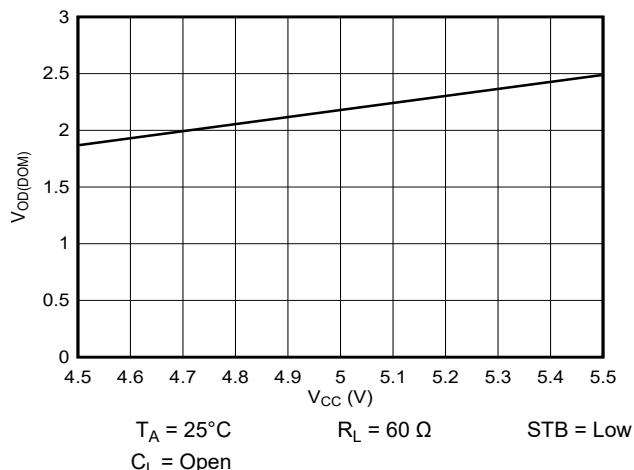
Figure 8-2. V_{OD(DOM)} over V_{CC}
