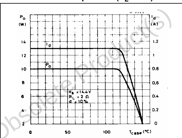
Figure 25. Output power and drain current vs. case temperature ( R_L = 2 \Omega )
