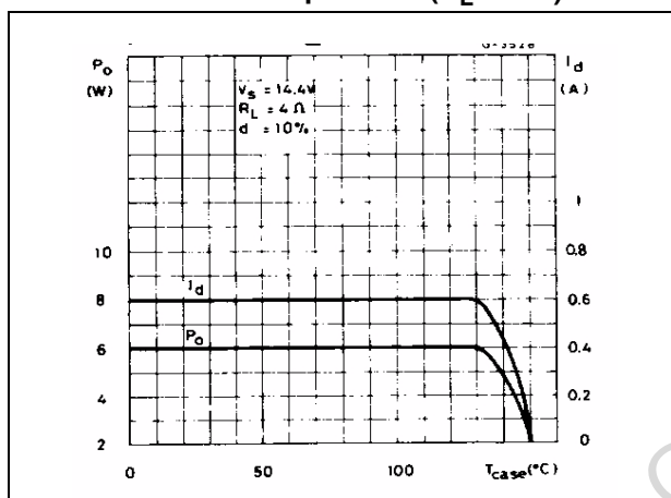
Figure 24. Output power and drain current vs. case temperature ( R_L = 4 \Omega )
