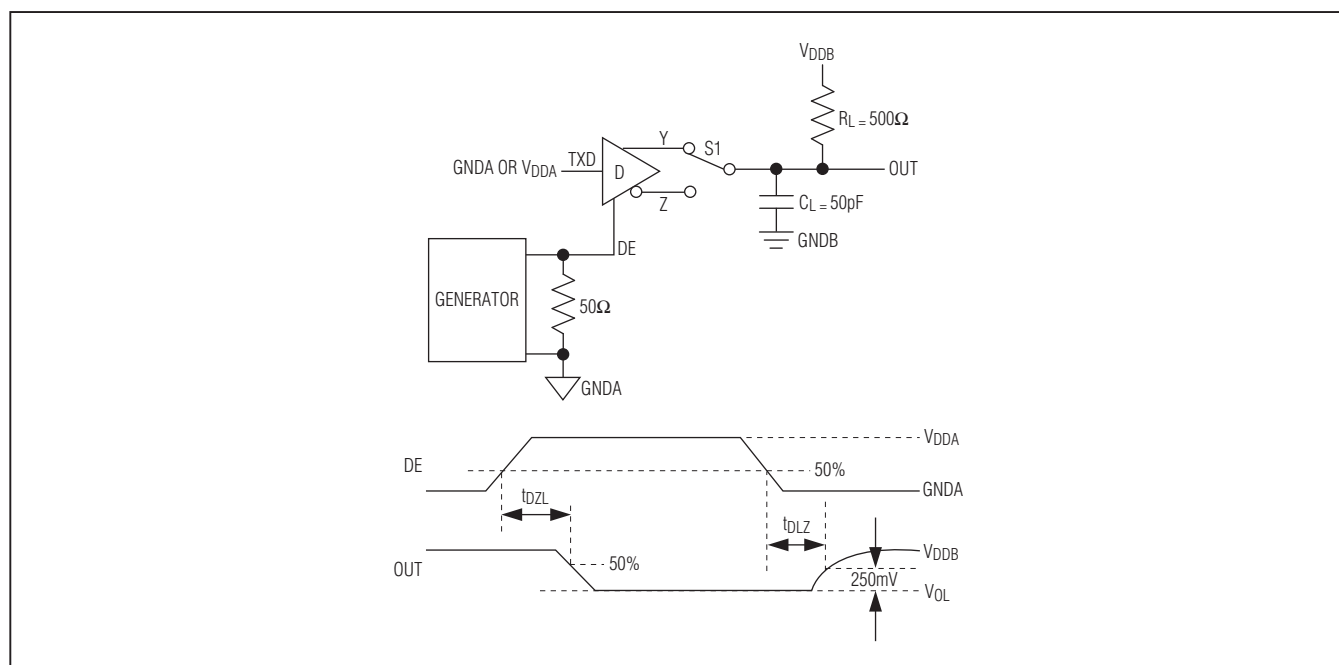
Figure 5. Driver Enable and Disable Times ( t_{DZL} , t_{DLZ} )
