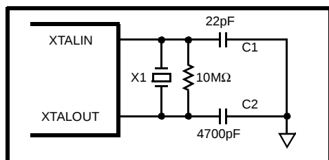
FIGURE 11. 32.768kHz CRYSTAL
