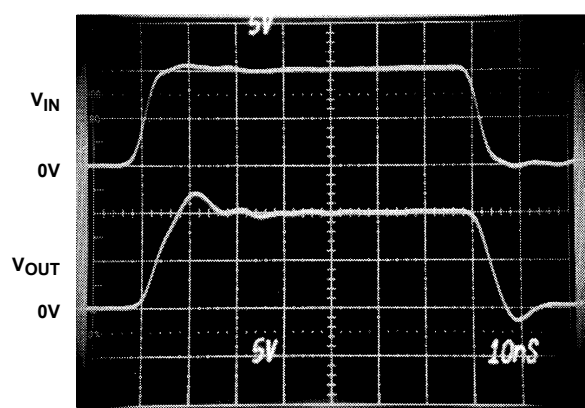
+10V RESPONSE
