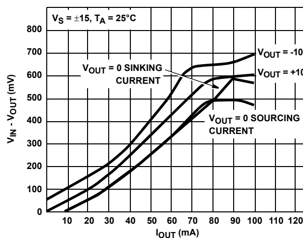
FIGURE 17. V_{IN} - V_{OUT} vs I_{OUT}
