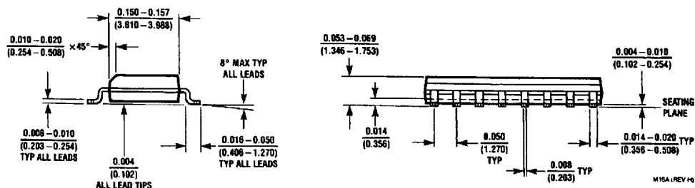
16-Lead Small Outline Molded Package (M) Order Number DM74LS173AM NS Package Number M16A
