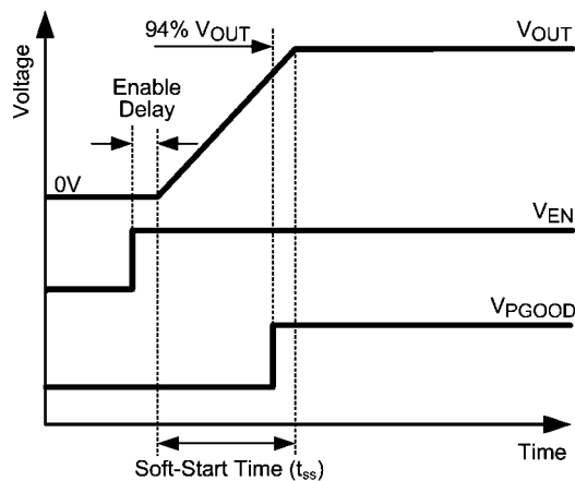
FIGURE 7. Soft-Start Timing
