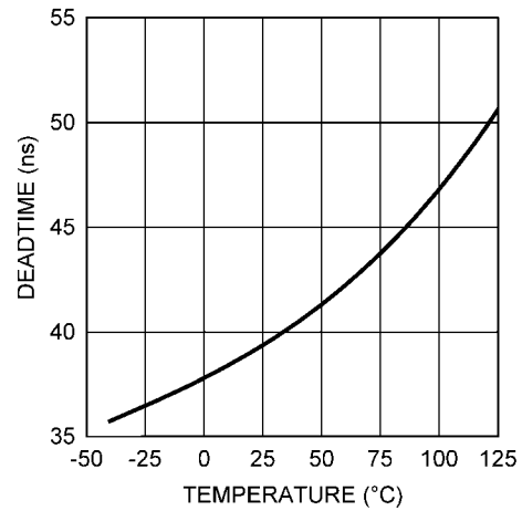
Deadtime vs Temperature
