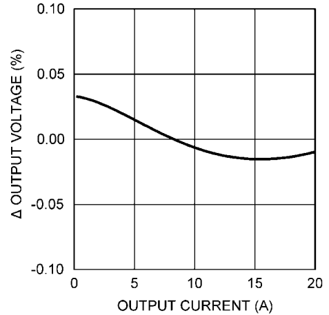
Load Regulation ( V_{out} = 1.5V )
