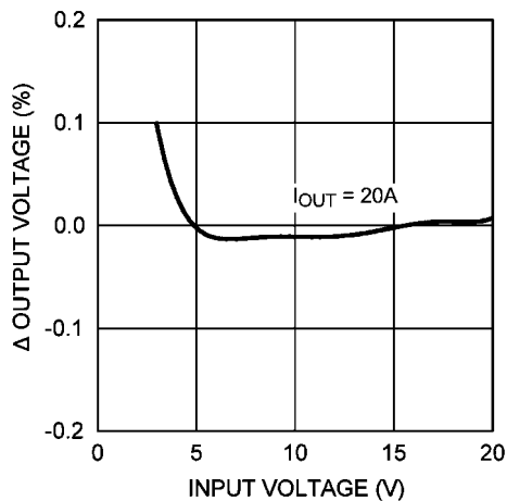
Line Regulation ( V_{out} = 1.5V )
