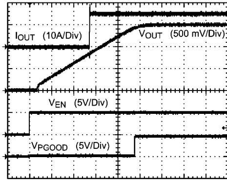
Startup Waveforms
