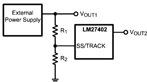
FIGURE 8. Tracking an External Power Supply
