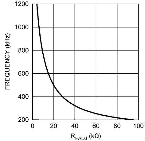
Frequency vs R_{FADJ}
