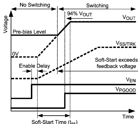
FIGURE 1. Pre-Bias Startup
