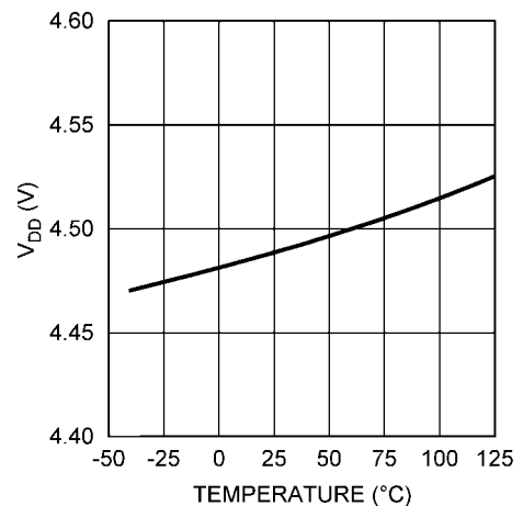
VDD Voltage vs Temperature ( I_{VDD} = 25mA )
