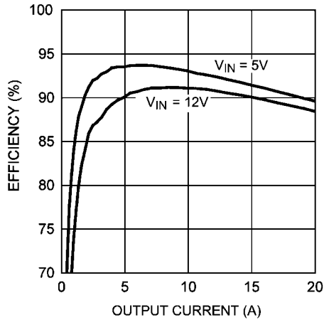
Efficiency ( V_{out} = 1.5V )
