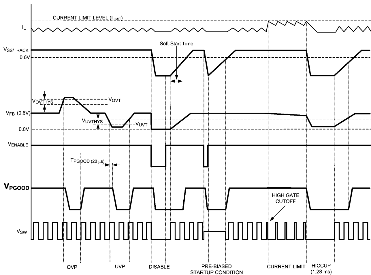
FIGURE 3. Power Good Behavior
