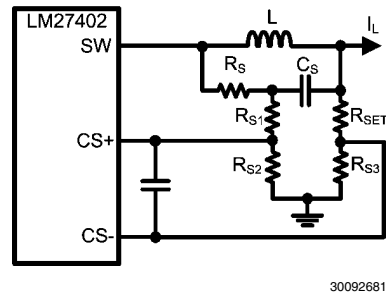
FIGURE 12. Common Mode Voltage Resistor Divider Network
