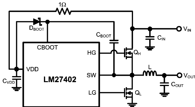
FIGURE 18. Tie V DD to V IN when VIN ≤ 5.5V
