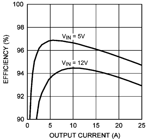
Efficiency ( V_{out} = 3.3V , Example Circuit 2)
