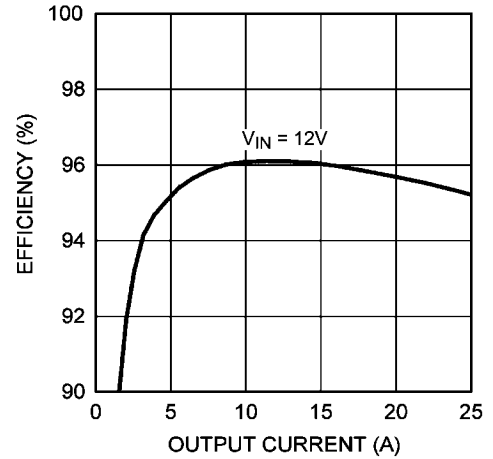
Efficiency ( V_{out} = 5V , Example Circuit 2)
