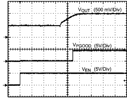
Pre-Bias Startup Waveforms
