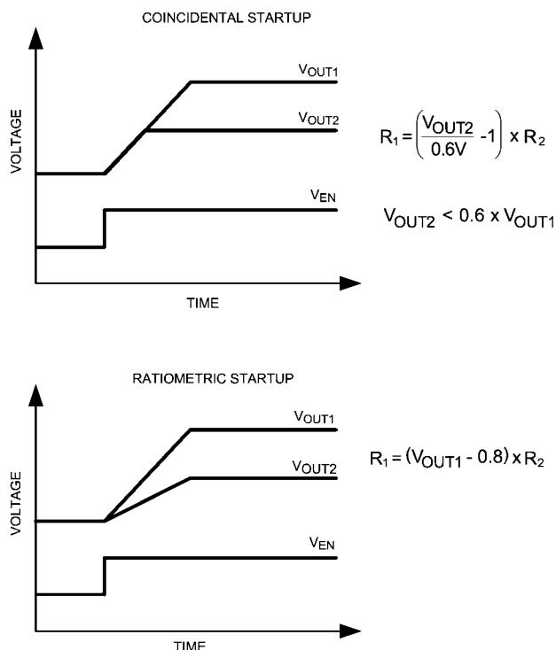
FIGURE 9. Tracking Startup Sequences
