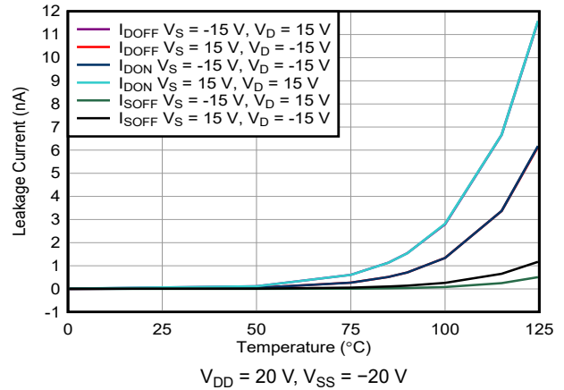
Figure 7-16. Leakage Current vs Temperature
