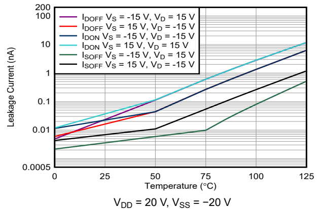
Figure 7-18. Leakage Current vs Temperature
