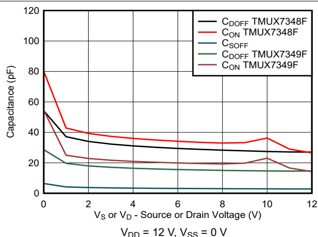
Figure 7-34. Capacitance vs Source or Drain Voltage
