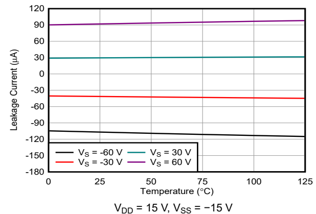
Figure 7-23. I_{S(FA)} Overvoltage Leakage Current vs Temperature
