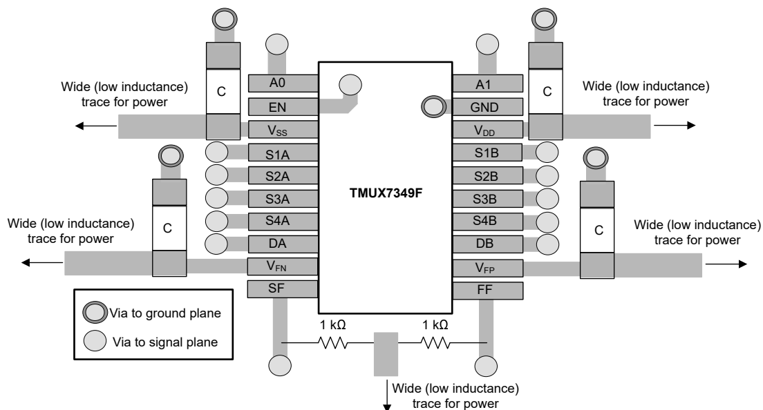
Figure 10-5. TMUX7349FPW Layout Example
