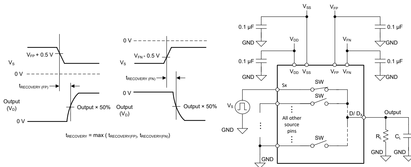
Figure 8-10. Fault Recovery Time Measurement Setup
