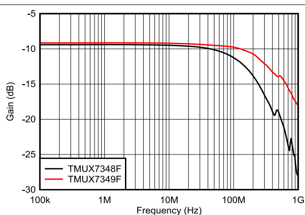
Figure 7-32. On Response vs Frequency
