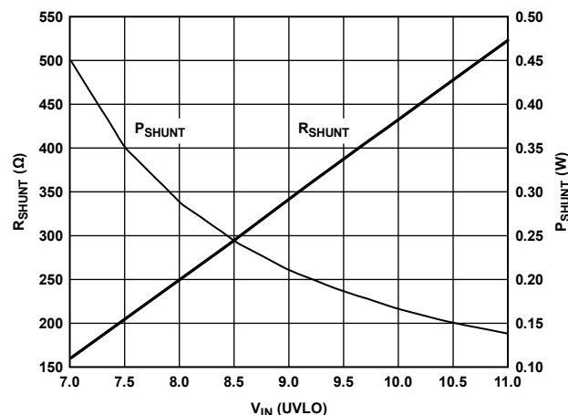
Figure 14. Typical Shunt Resistor Value and Power Dissipation for Different UVLO Voltages
