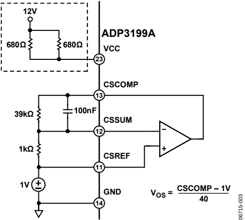
Figure 5. Current Sense Amplifier Offset Voltage (V OS )
