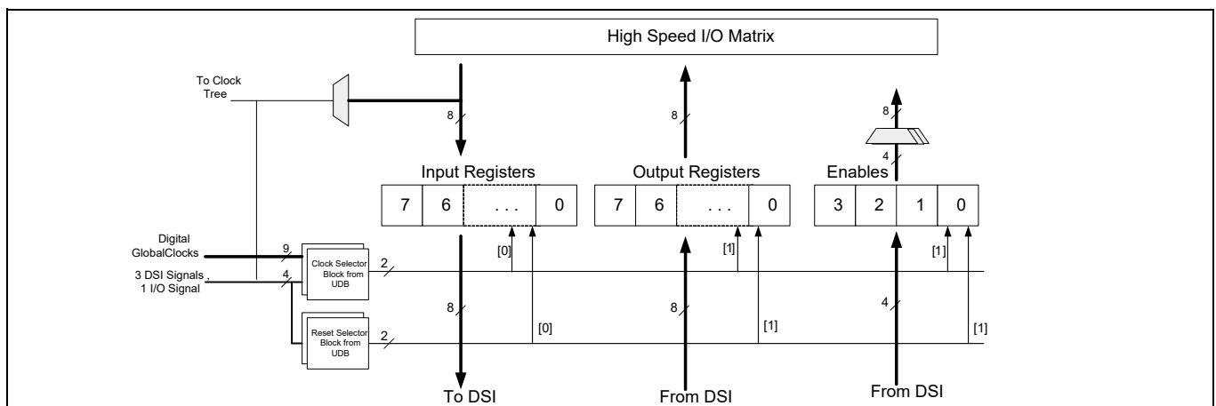
Figure 7 Port interface
