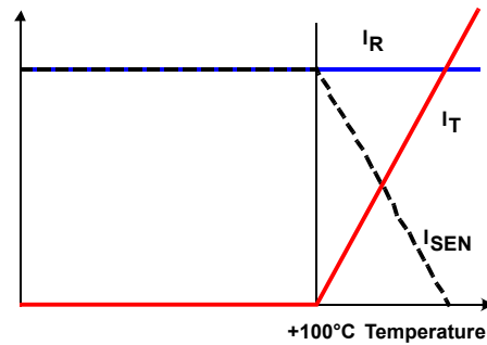
Figure 22. Current Signals at the Amplifier CA Input
