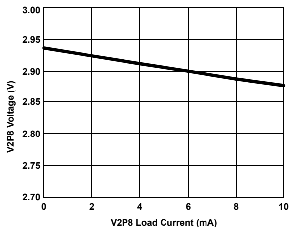
Figure 10. V2P8 Output vs Load Current
