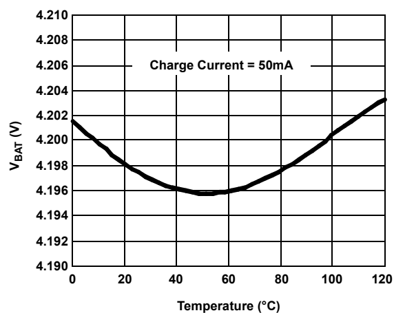
Figure 4. Charger Output Voltage vs Temperature
