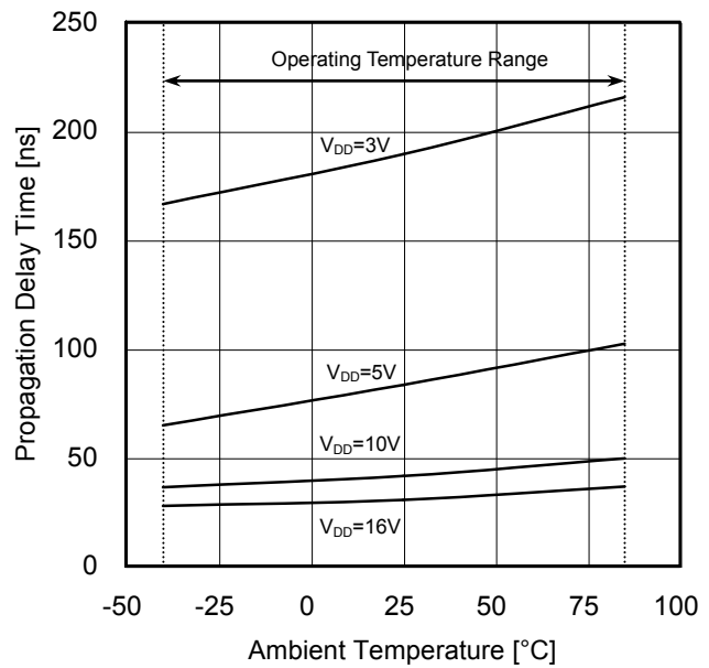
Figure 10. "H" to "L" Propagation Delay Time t_{PHL}
