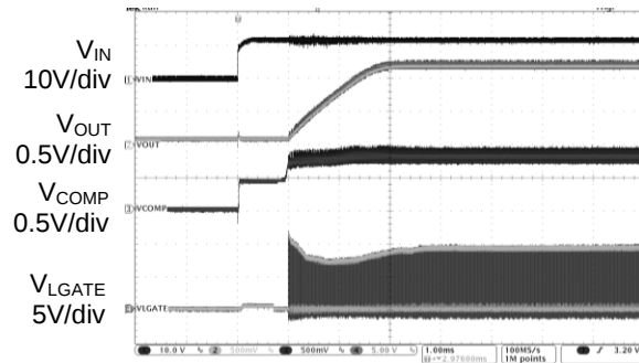
Power-on Waveform ( V_{IN}=12V , V_{OUT}=1.2V , I_{OUT}=0A )
