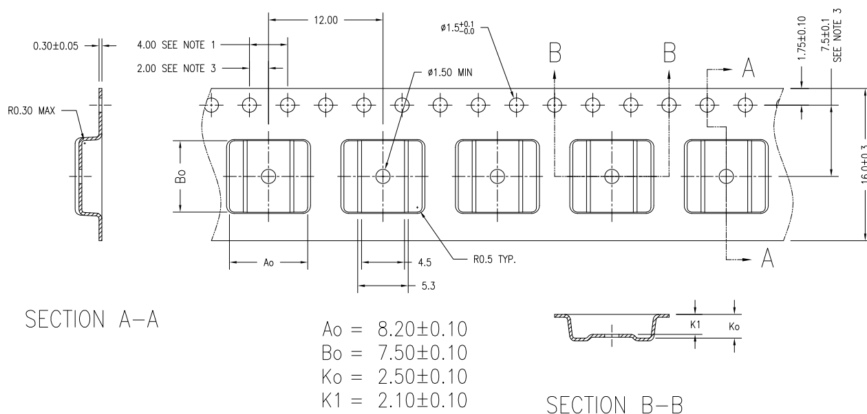
Figure 11. 20-pin SSOP (209 Mils) Advantek Carrier Tape Drawing, 51-51101
