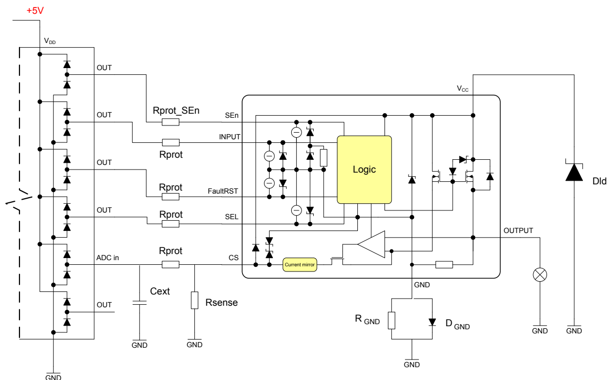
Figure 12. Application diagram
