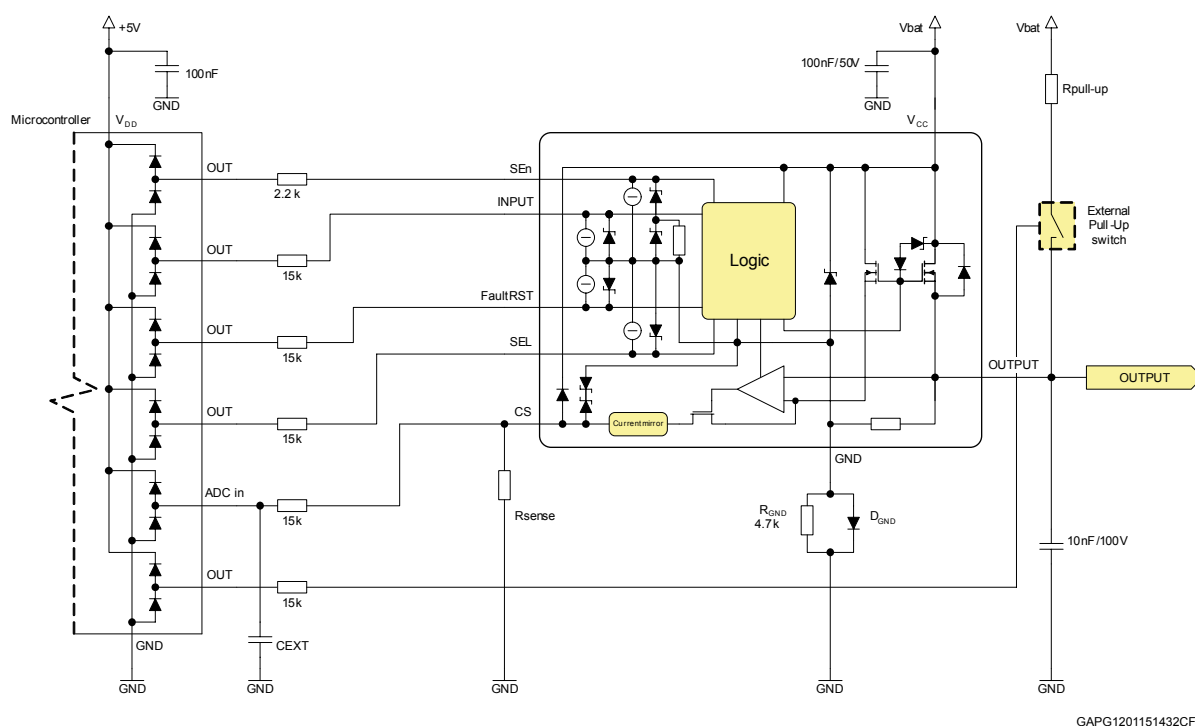
Figure 18. Open-load / short to V_{CC} condition
