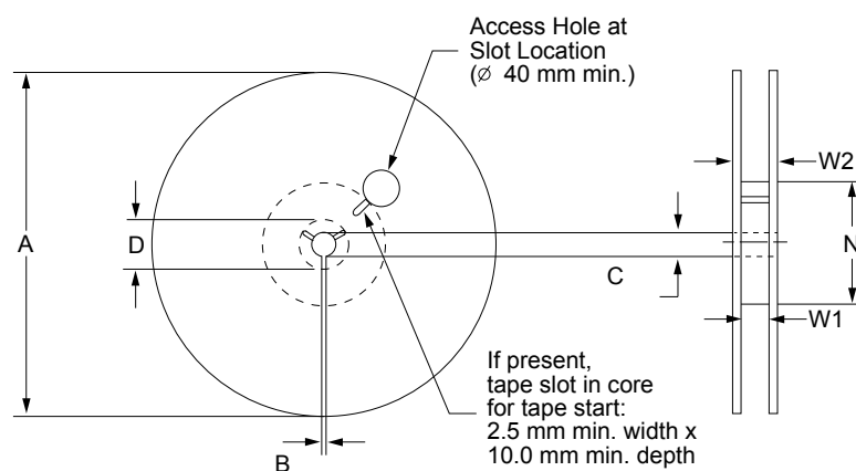
Figure 28. PowerSSO-16 reel 13"
