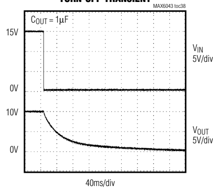
TURN-OFF TRANSIENT
