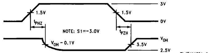
FIGURE 6. Receiver TRI-STATE Timing ( t_{PHZ} , t_{PZH} )
