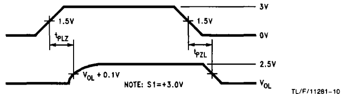
FIGURE 7. Receiver TRI-STATE Timing ( t_{PLZ} , t_{PZL} )
