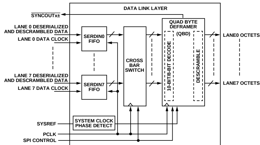
Figure 48. Data Link Layer Block Diagram
