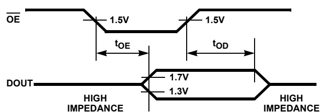
FIGURE 6. OUTPUT ENABLE, DISABLE TIMING
