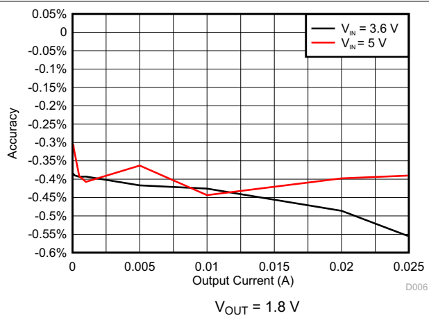
Figure 6-6. DCDC6 Accuracy
