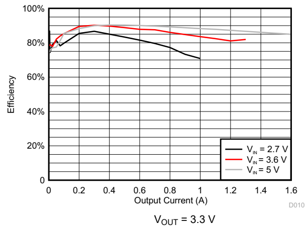
Figure 8-6. DCDC4 Efficiency
