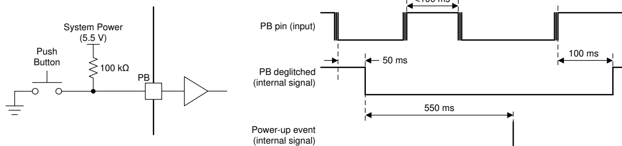
Figure 7-26. Left: Typical PB Input Circuit Right: Push-Button Input (PB) Deglitch and Power-Up Timing
