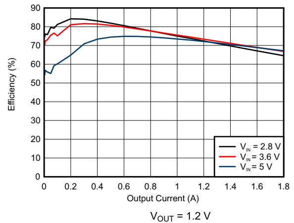
Figure 8-4. DCDC3 Efficiency
