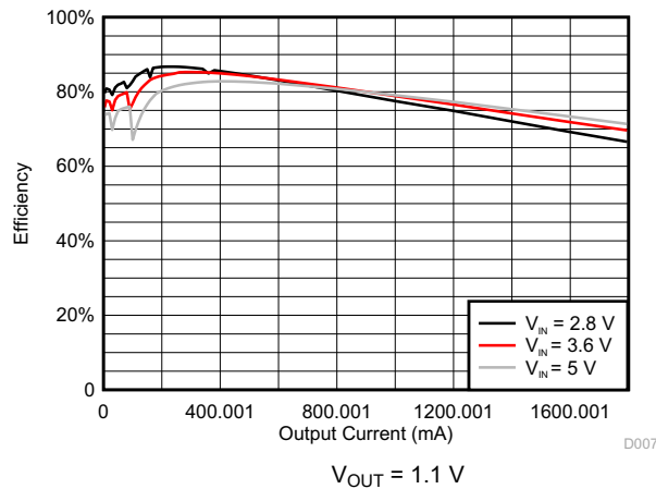
Figure 8-3. DCDC1/DCDC2 Efficiency
