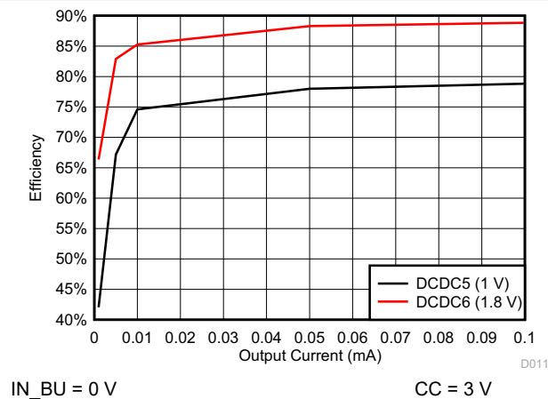
Figure 8-7. DCDC5/DCDC6 Efficiency
