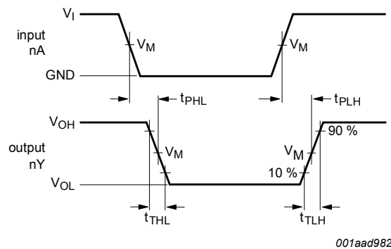
Fig. 5. Propagation delays data input (nA) to output (nY)
