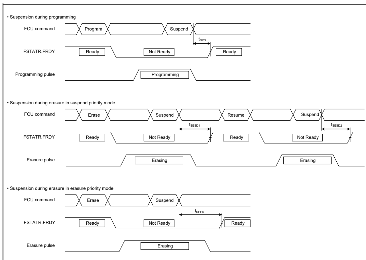
Figure 5.82 Flash Memory Programming/Erasure Suspension Timing
