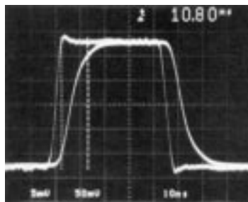
LT1194 • TPC20 RISE TIME = 10.8ns, PROPAGATION DELAY = 6ns
