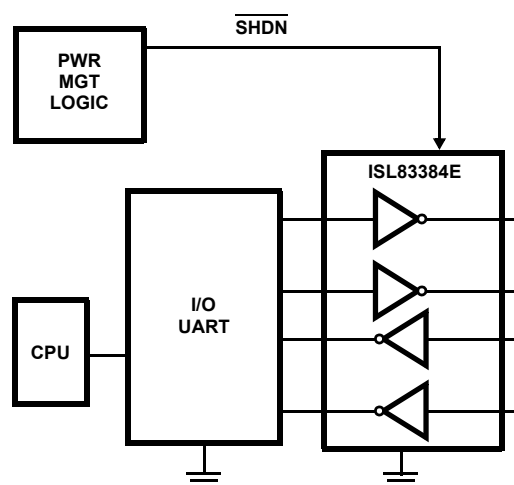
FIGURE 4. CONNECTIONS FOR MANUAL POWERDOWN
