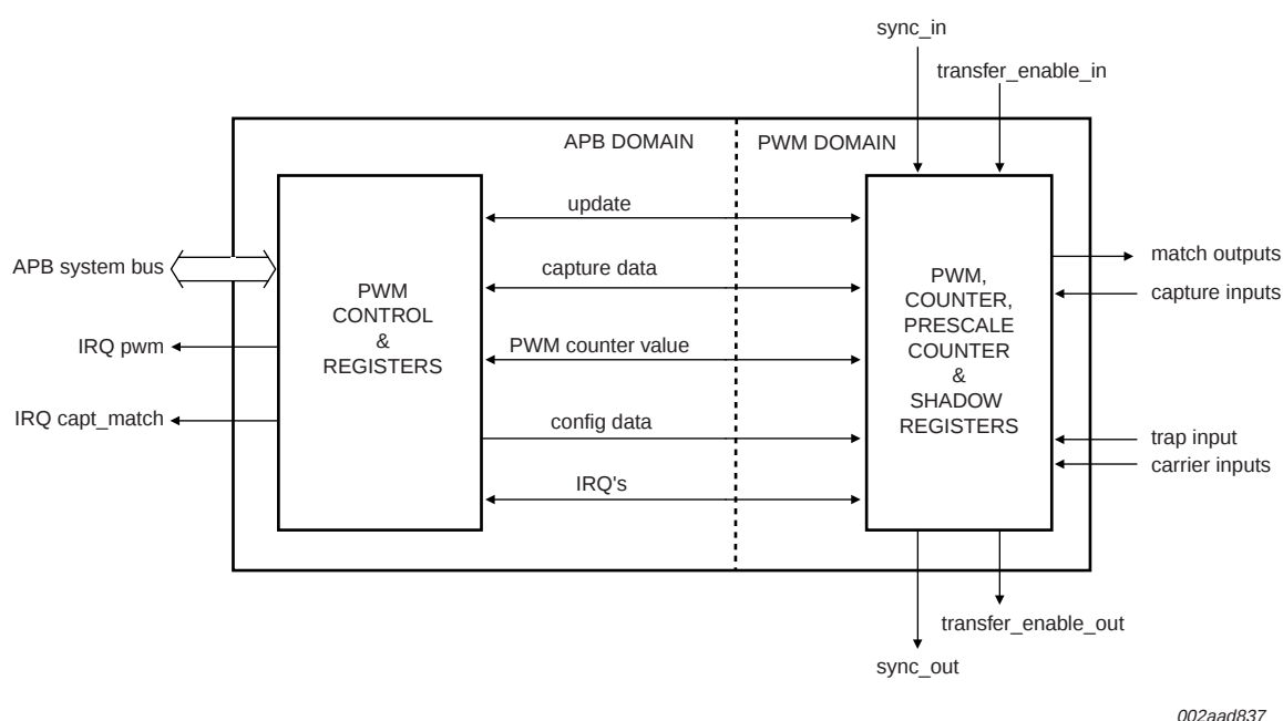
Fig 10. PWM block diagram
