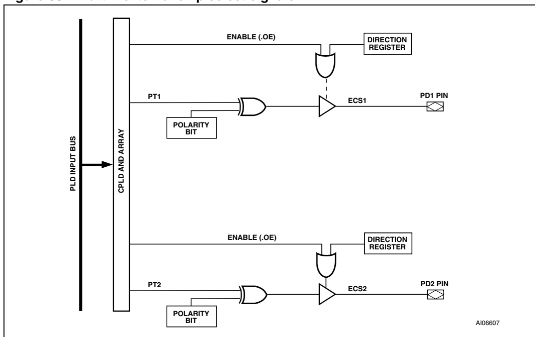
Figure 66. Port D external chip select signals
