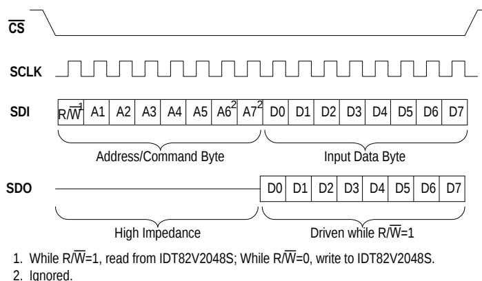
Figure-21 Serial Host Mode Timing
