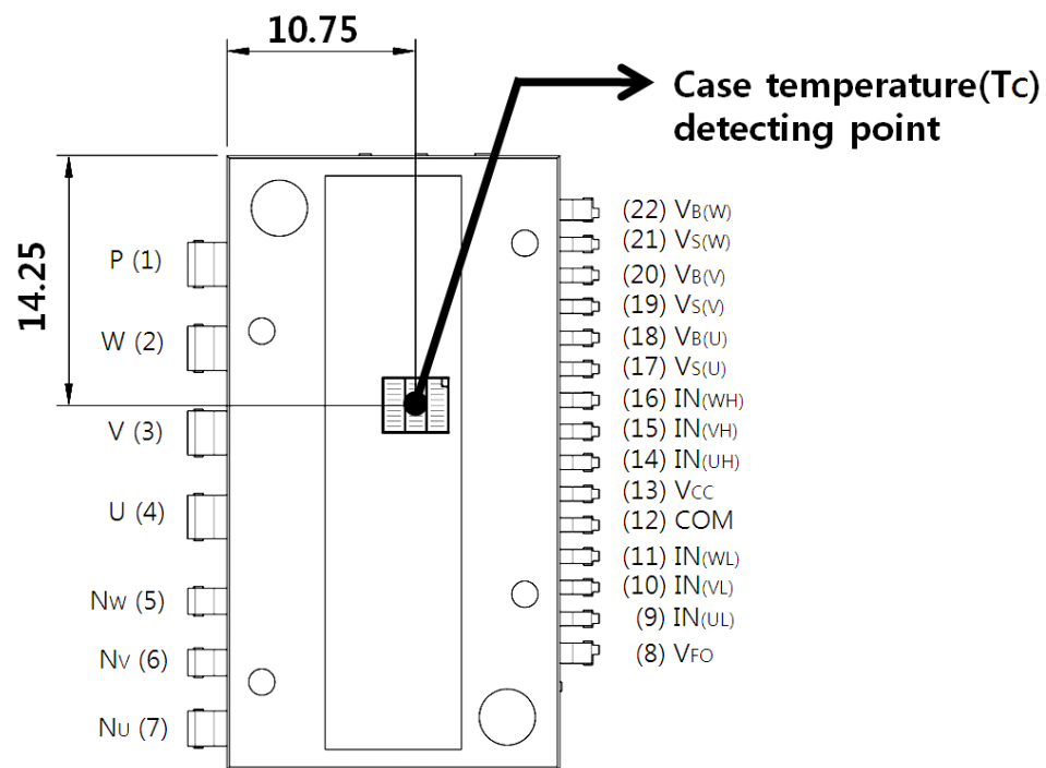
Figure 2.Top View
