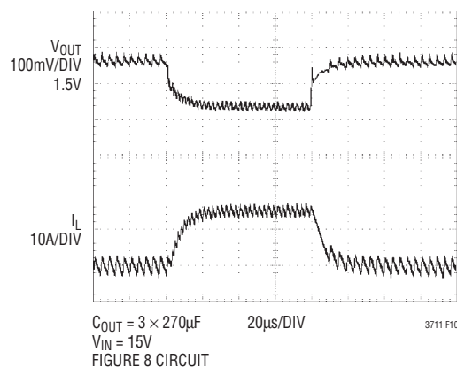
Figure 12. Transient Response with Active Voltage Positioning
