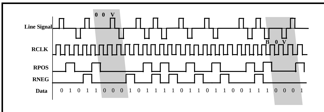
FIGURE 19. AN EXAMPLE OF B3ZS DECODING
