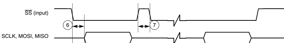
Figure 18. Slave CSPI Timing Diagram FIFO Advanced by \overline{\text{SS}} Rising Edge
