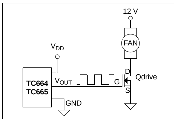
FIGURE 4-3: PWM Fan Drive.
