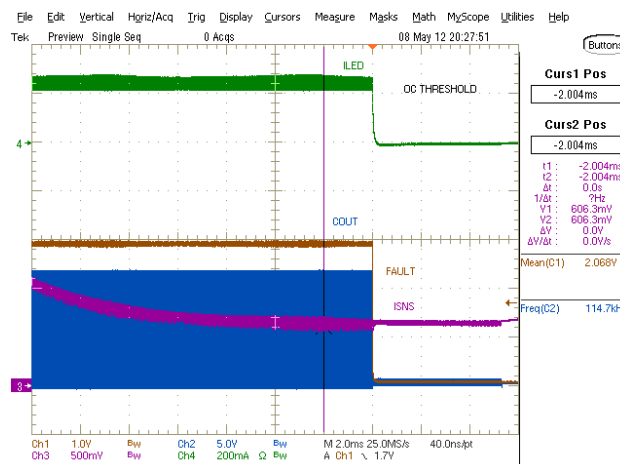
Figure 19 • OC Threshold
