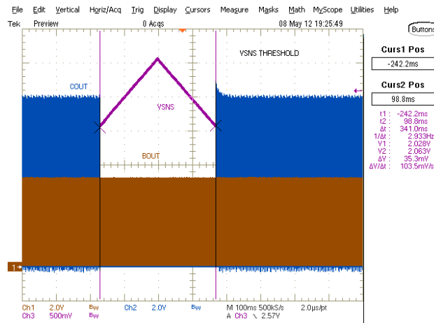
Figure 17 • VSNS Threshold
