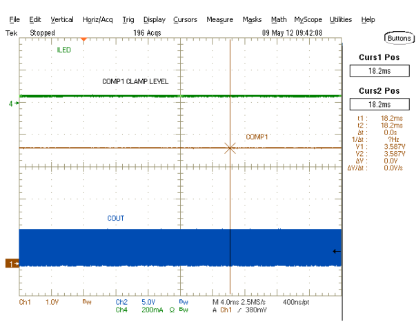
Figure 26 • COMP1 Clamp Level
