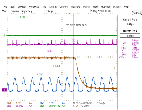
Figure 24 • FB1 OV Threshold
