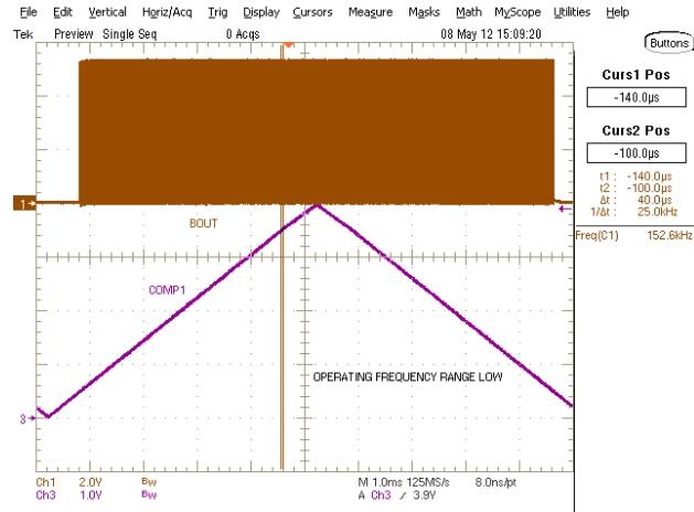
Figure 9 • Operating Frequency Range Low
