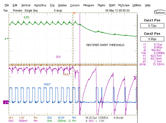
Figure 23 • Rectifier Short Threshold
