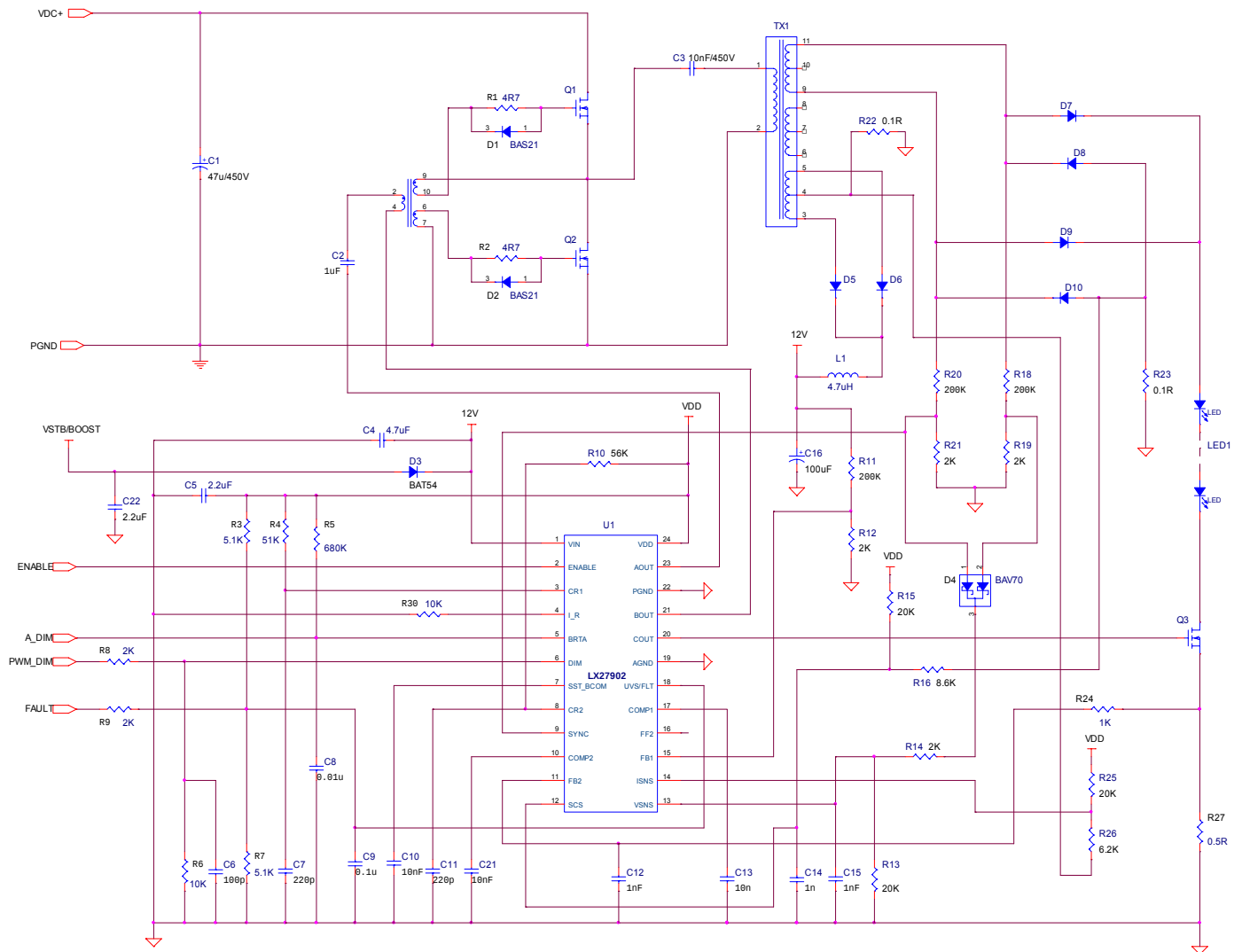
Figure 27 • Application Schematic
