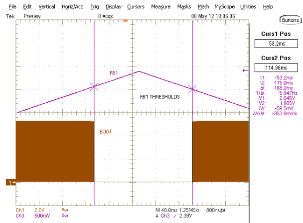
Figure 16 • FB1 Thresholds
