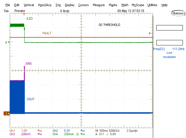
Figure 20 • OC Threshold
