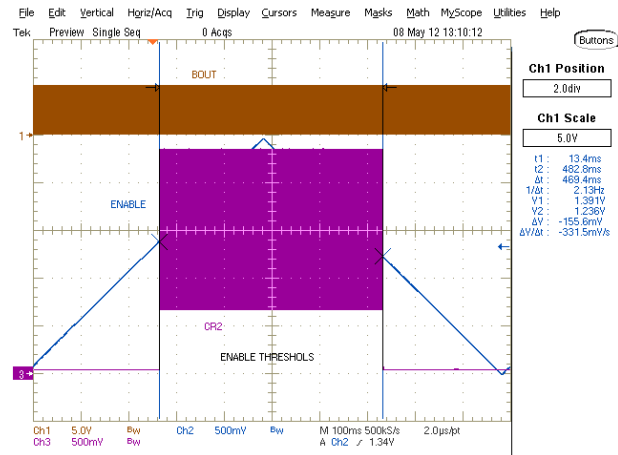
Figure 3 • Enable Threshold
