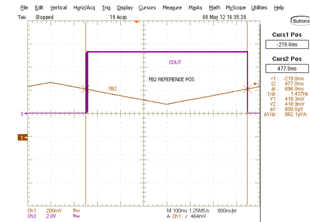
Figure 11 • FB2 Reference Positive
