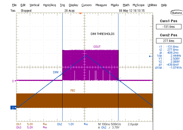
Figure 13 • Dim Thresholds
