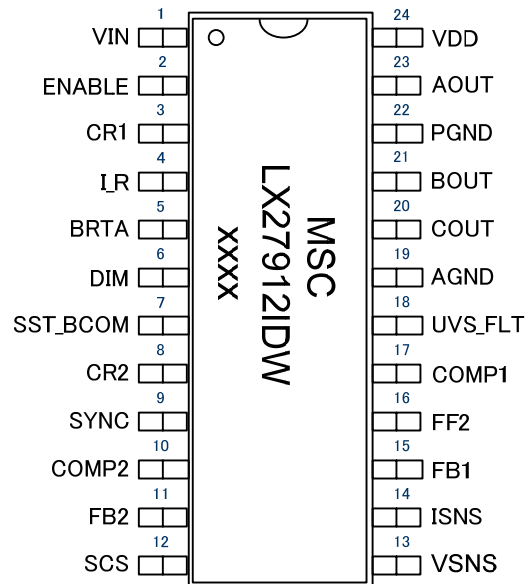
Figure 2 • Pinout
