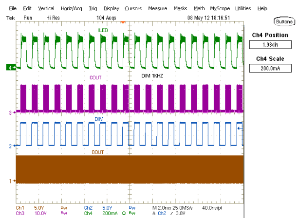
Figure 14 • DIM 1kHz
