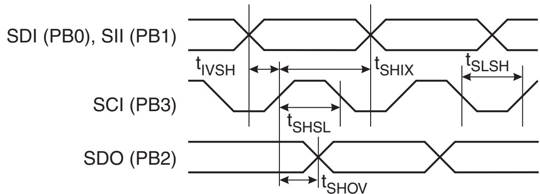
Figure 18-5. High-voltage Serial Programming Timing
