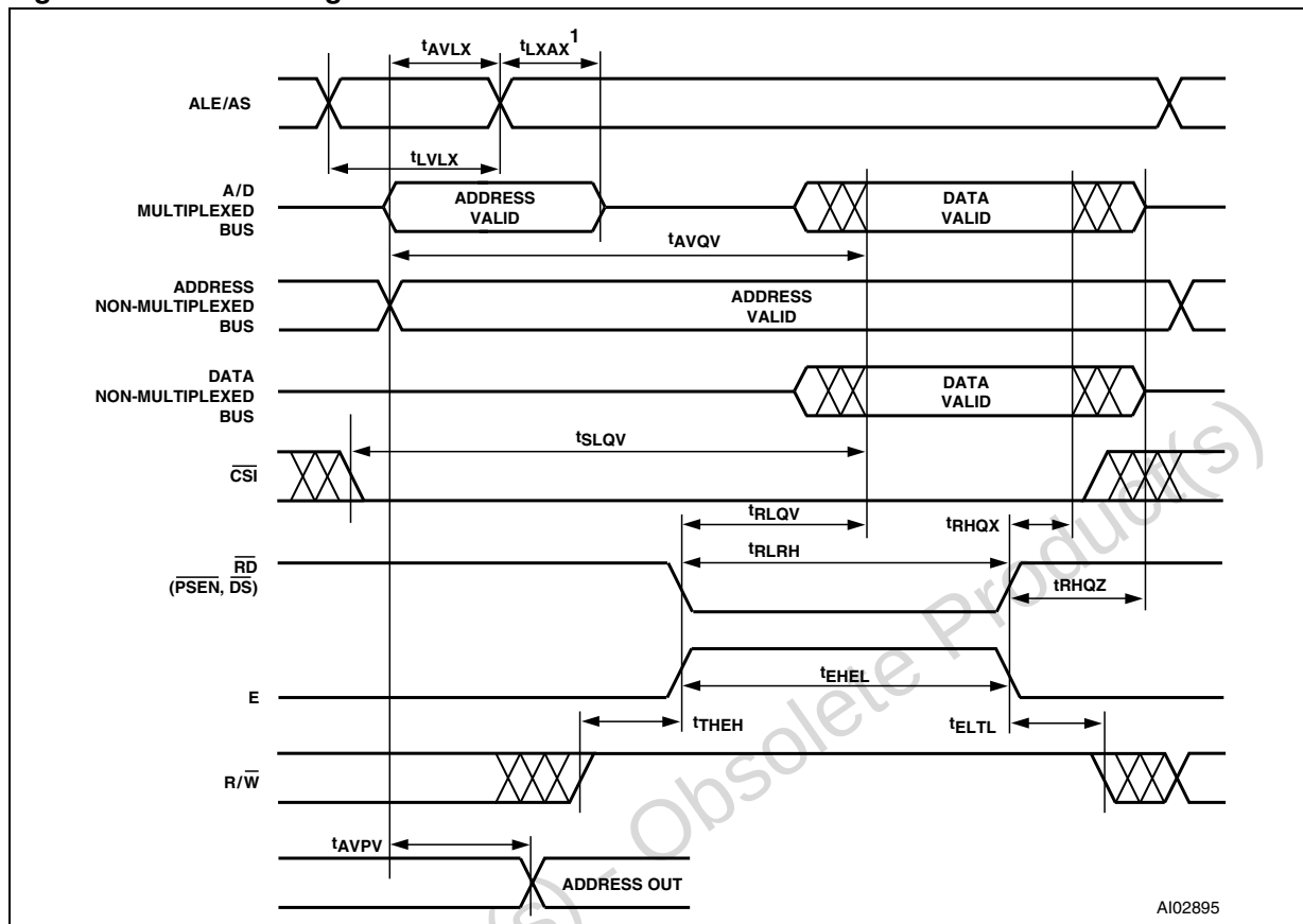
Figure 43. READ timing
