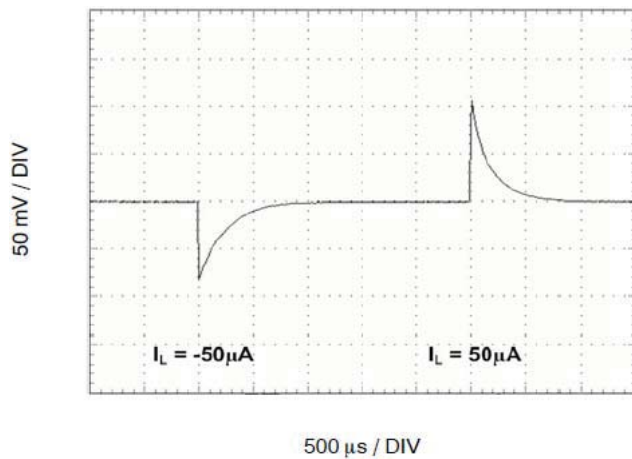
Figure 12. Load Transient ( I_L = 50\mu\text{A} )
