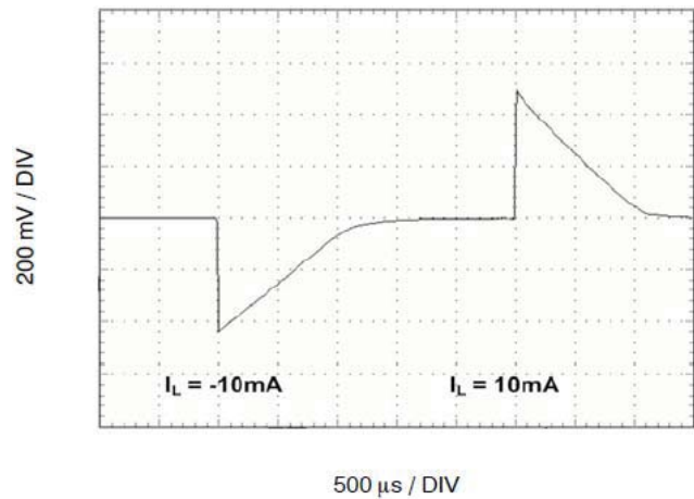
Figure 13. Load Transient ( I_L = 10\text{mA} )
