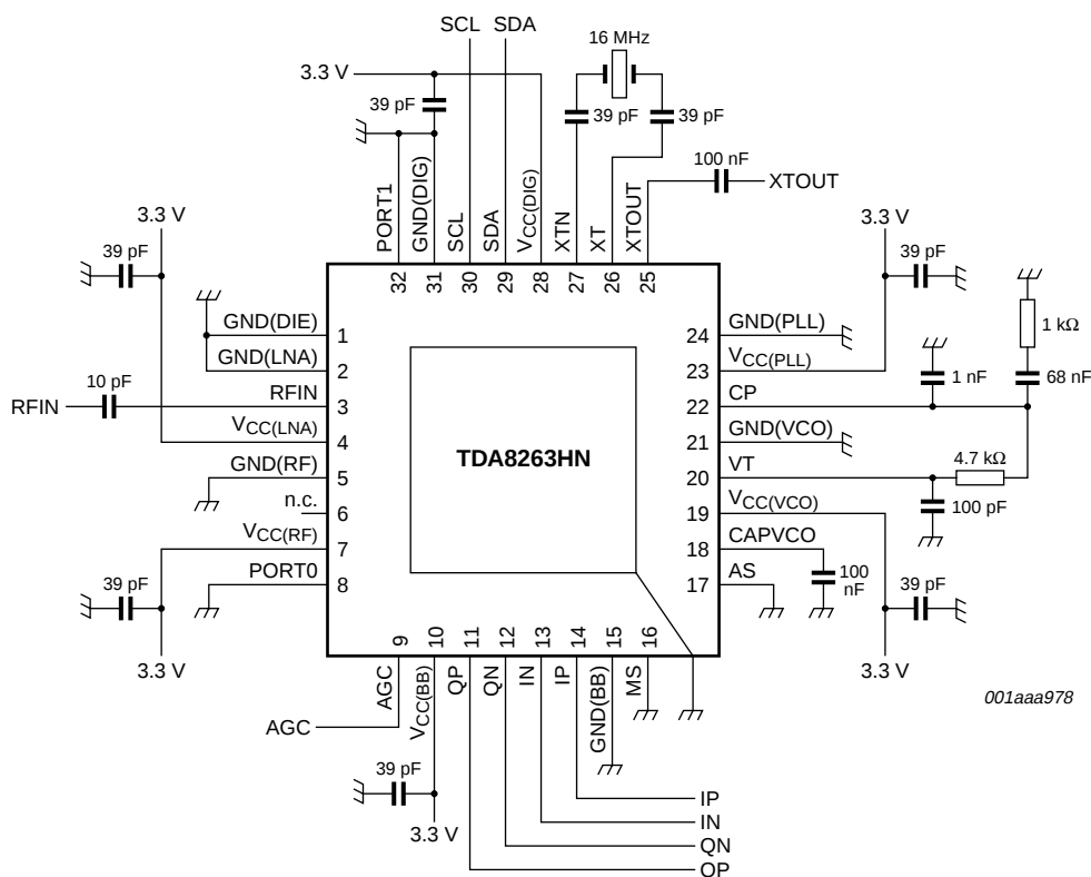
Fig 6. Typical application circuit
