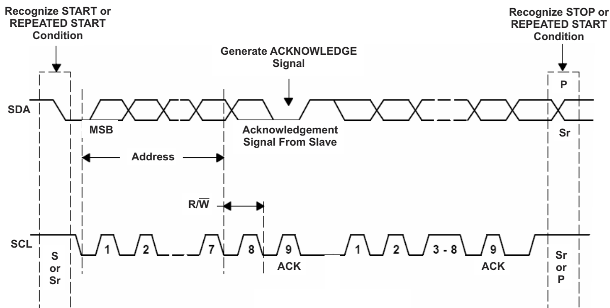
Figure 8-9. Bus Protocol
