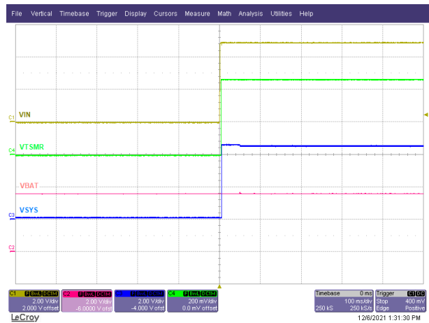
Figure 9-3. Power Up from Shutdown Mode with VIN Supply Insertion
