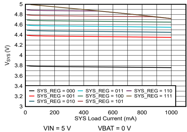
Figure 7-4. SYS Load Regulation
