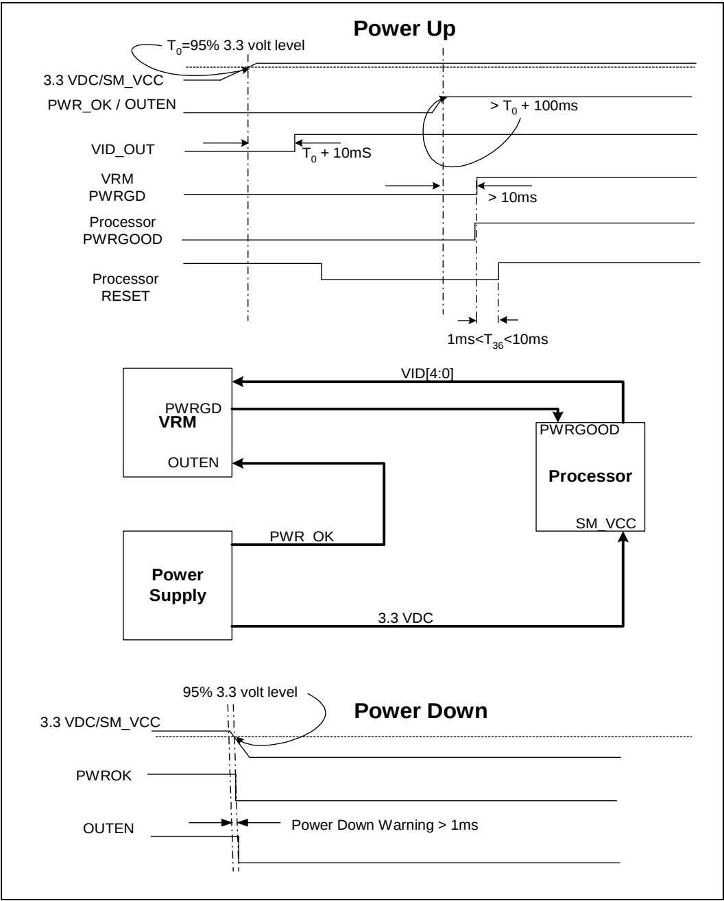
Figure 19. Example 3.3 VDC/SM_VCC Sequencing
