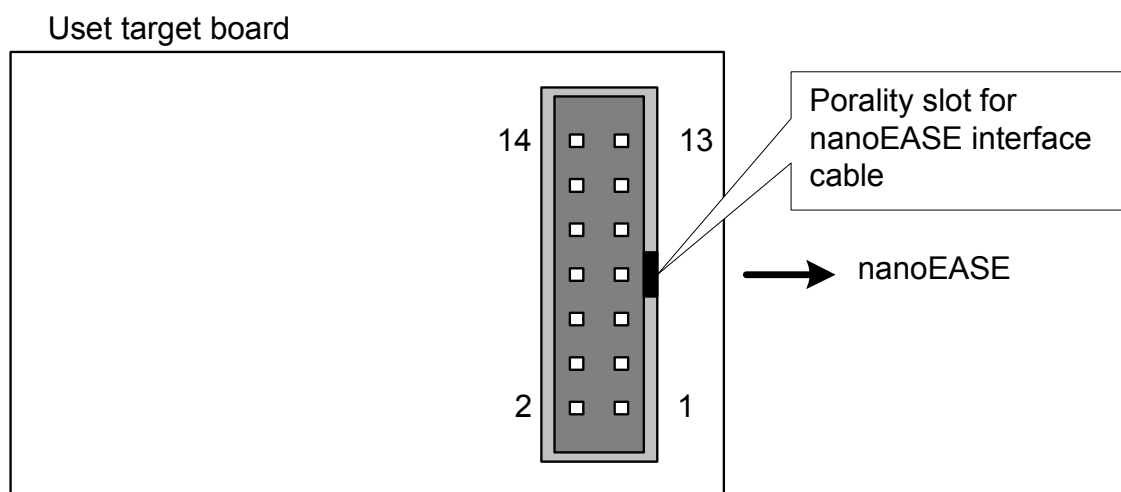
Fig 7 recommended board layout of nanoEASE interface socket
