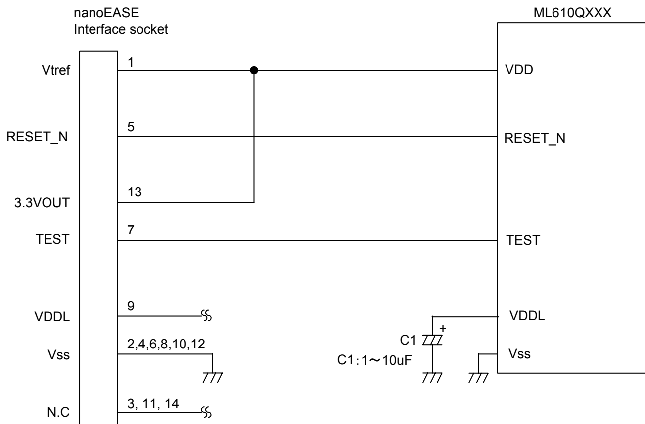
Fig 6 Recommended circuitry does not use VDDL terminal
