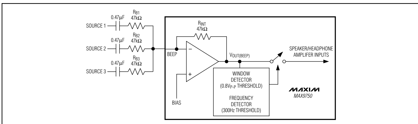
Figure 8. BEEP Input
