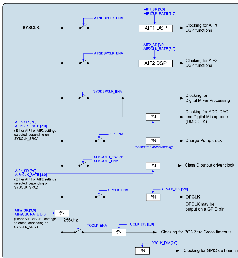
Figure 68 System Clocking
