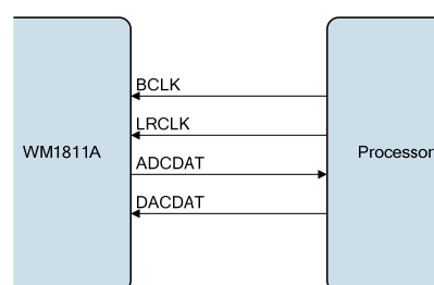
Figure 46 Slave Mode
