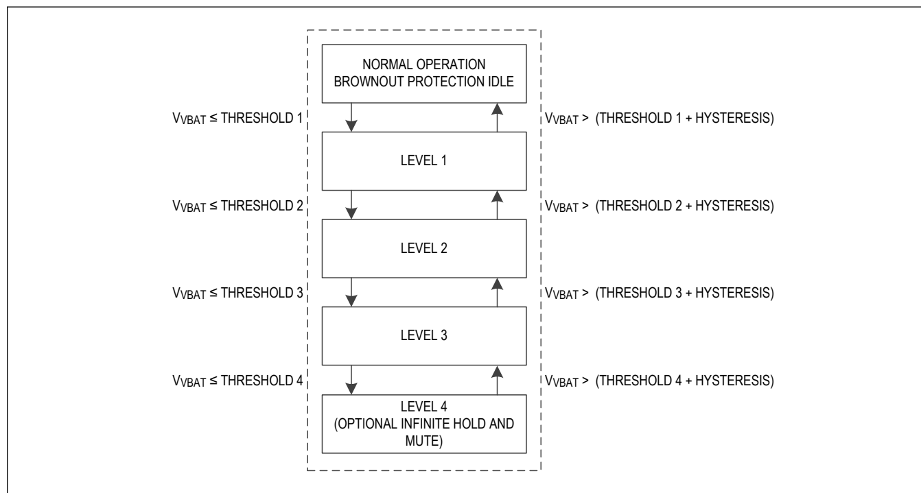
Figure 21. BDE Levels
