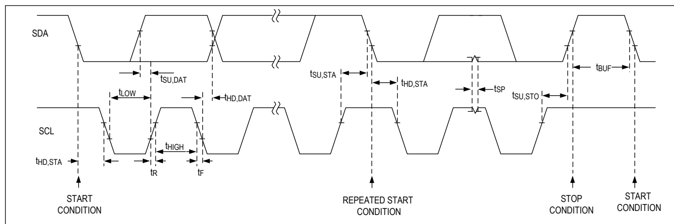
Figure 34. I^2C START, STOP, and REPEATED START Conditions
