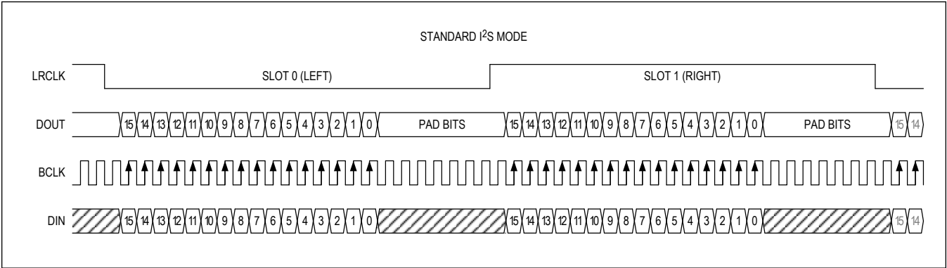
Figure 12. I 2 S Mode
