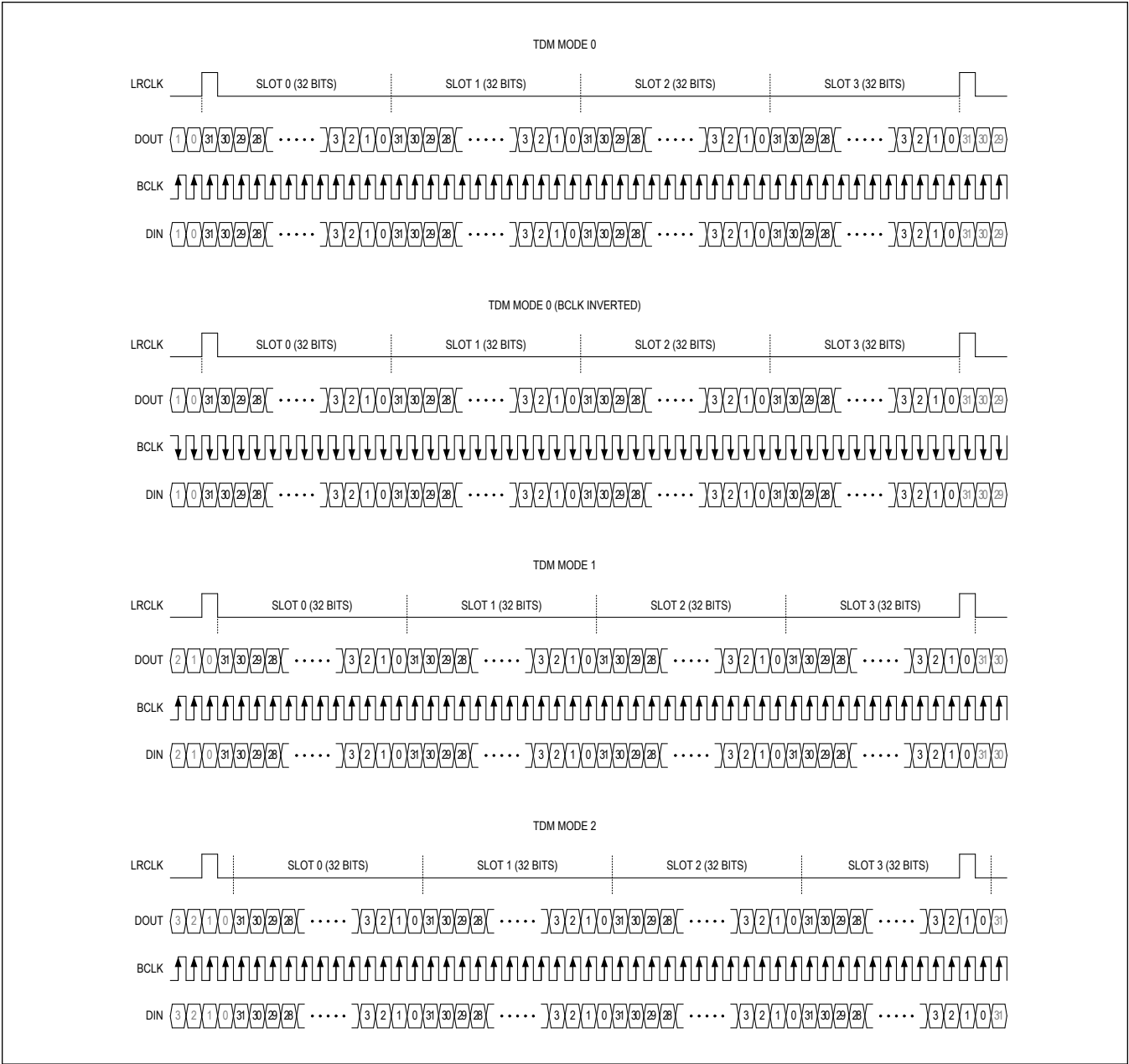
Figure 14. TDM Modes
