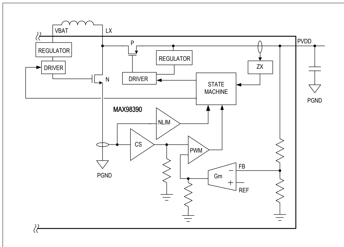
Figure 4. Boost Converter Block Diagram
