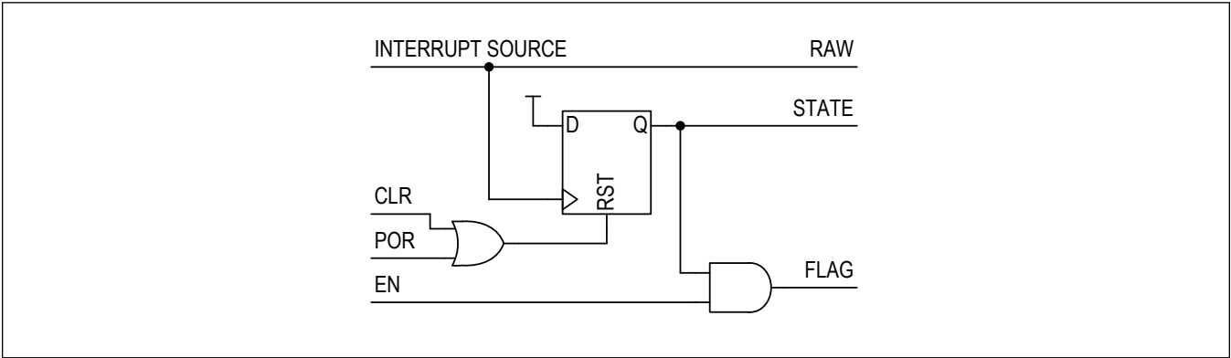
Figure 3. Interrupt Logic
