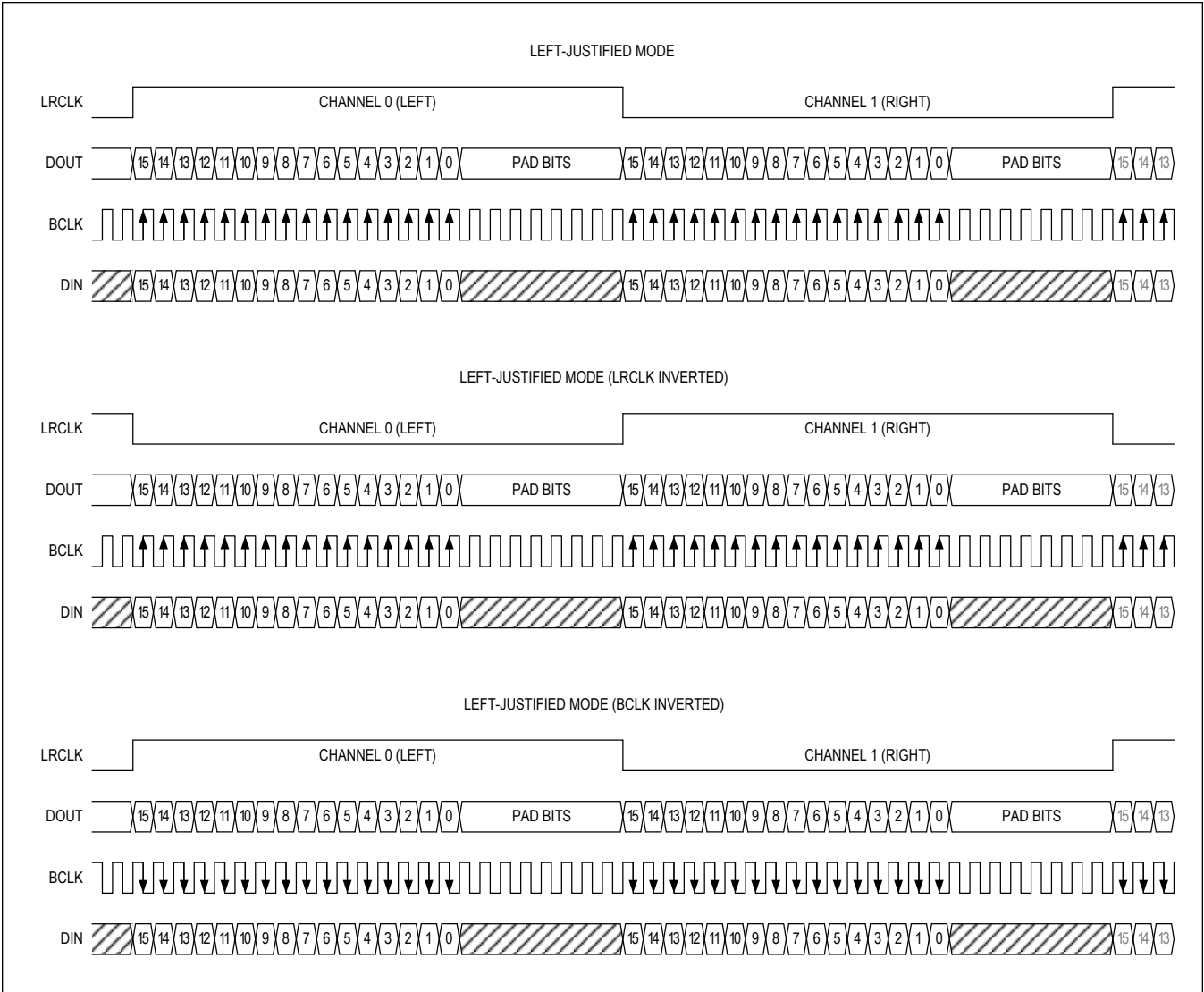
Figure 13. Left-Justified Modes
