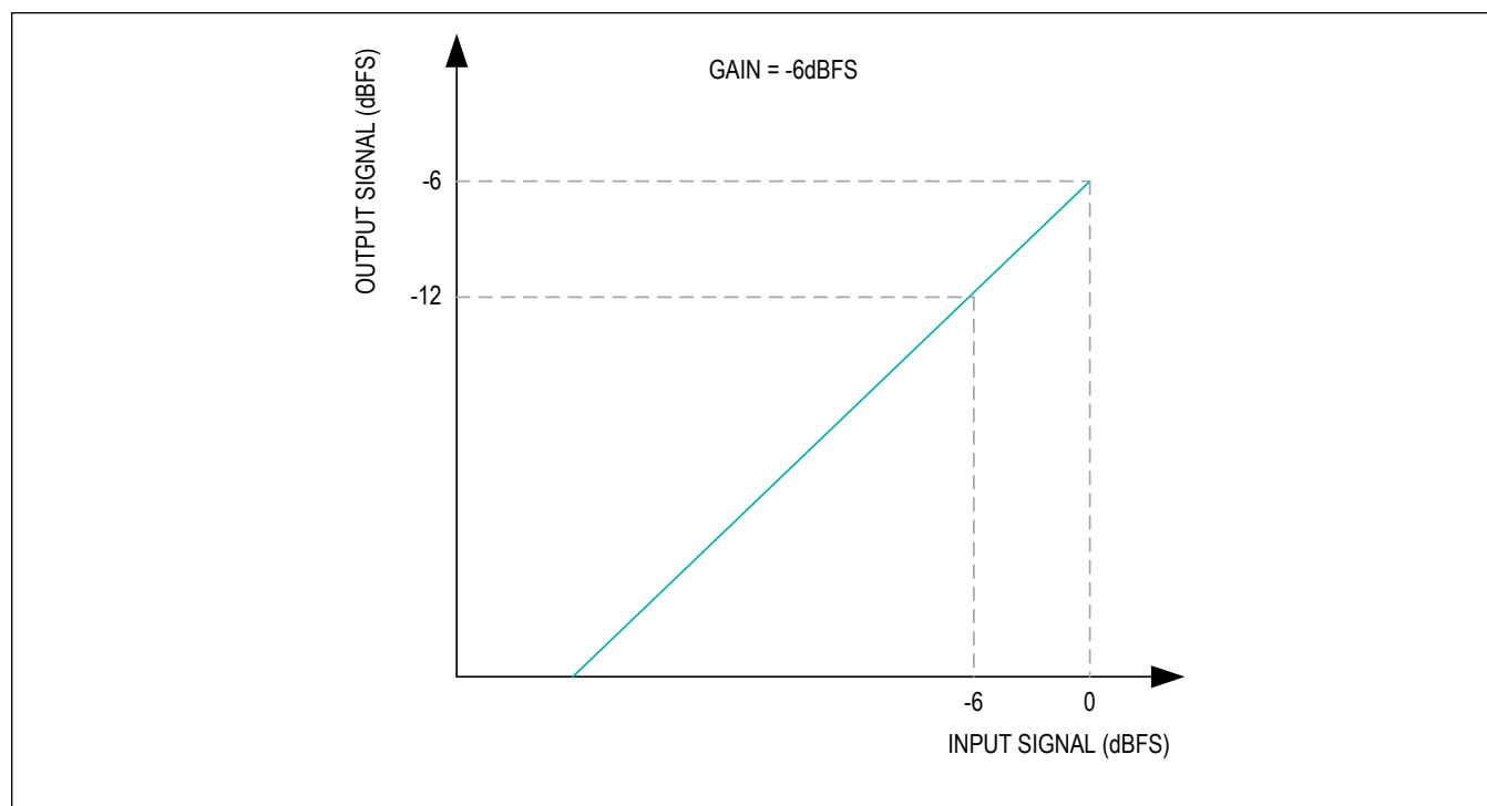
Figure 23. Gain Reduction Profile Example with -6dB Setting
