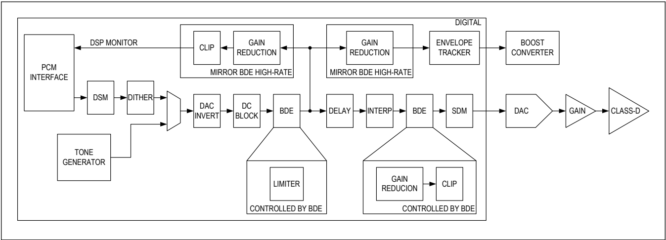
Figure 18. Amplifier Path
