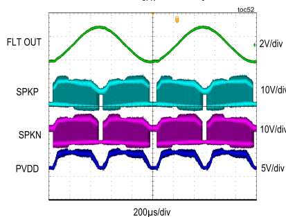
OUTPUT CLIPPING RESPONSE THD+N = 1%, Z_{SPK} = 4\Omega + 33\mu F
