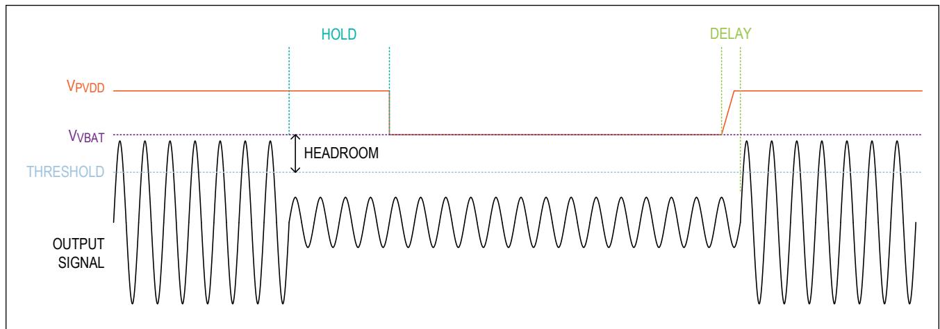
Figure 6. Boost Bypass
