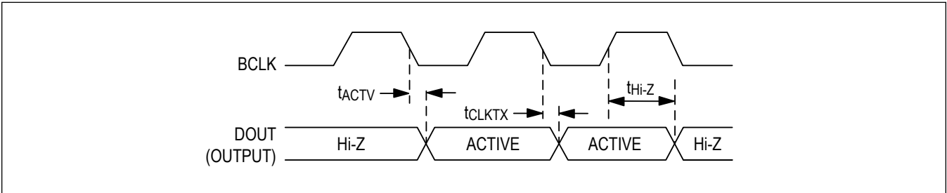
Figure 17. PCM Interface Timing/DOUT Timing Diagram
