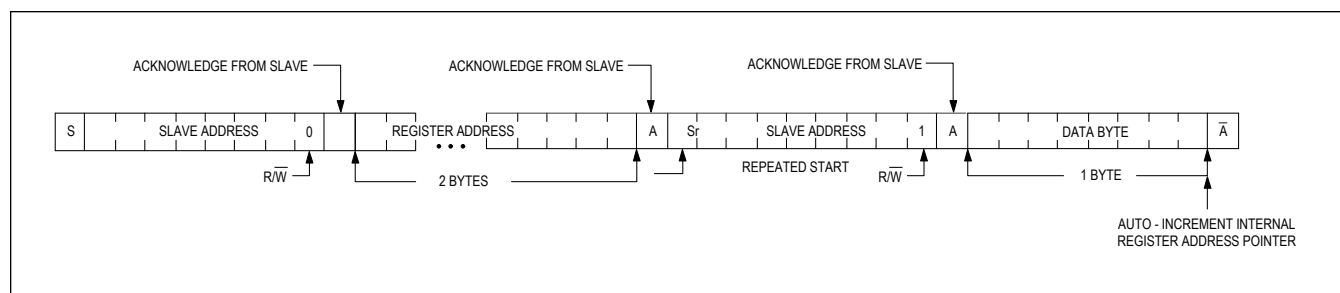
Figure 38. I 2 C Reading One Byte of Data from the Slave
