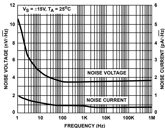
FIGURE 6. NOISE CHARACTERISTICS
