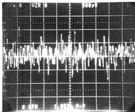
A_{\text{CL}} = 25,000\text{V/V} Horizontal Scale = 1\text{s/Div.} Vertical Scale = 0.002\mu\text{V/Div.} , E_N = 0.08\mu\text{V}_{\text{P-P RTI}} FIGURE 18. PEAK-TO-PEAK NOISE VOLTAGE (0.1Hz TO 10Hz)
