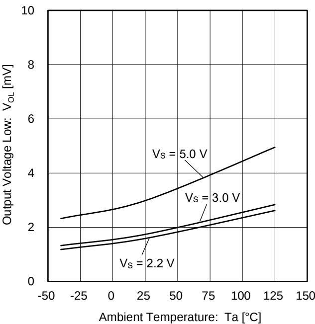
Figure 6. Output Voltage Low vs Ambient Temperature ( R_L = 10\text{ k}\Omega )
