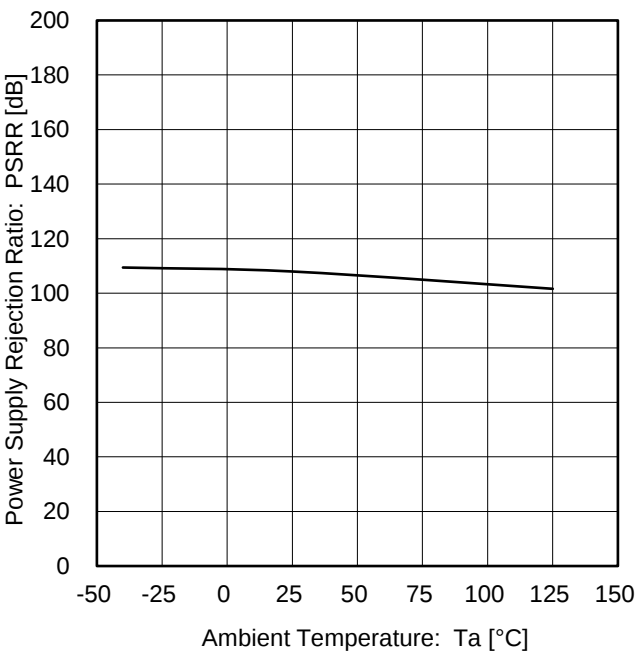
Figure 16. Power Supply Rejection Ratio vs Ambient Temperature
