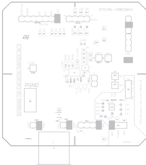
Figure 14: Top overlay
