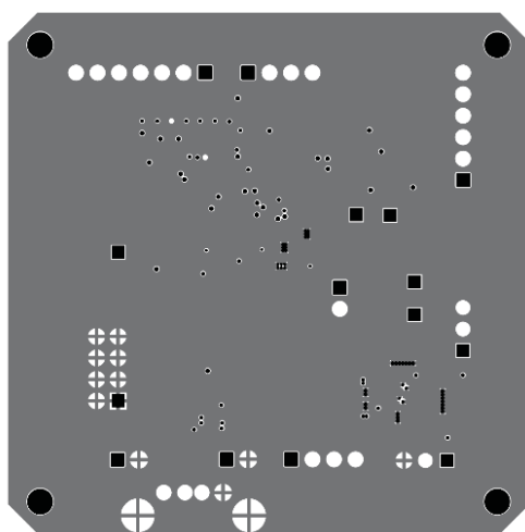
Figure 18: Bottom layer
