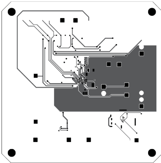
Figure 16: Mid layer 1
