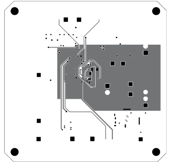
Figure 17: Mid layer 2
