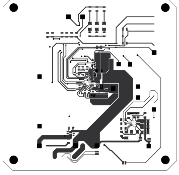
Figure 15: Top layer
