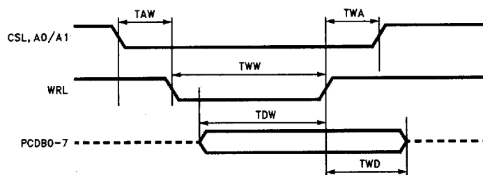
Figure 4. Host-Interface Write
