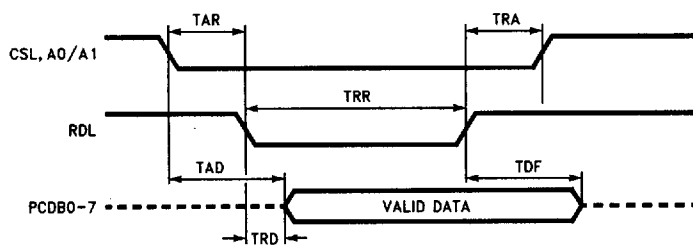
Figure 3. Host-Interface Read
