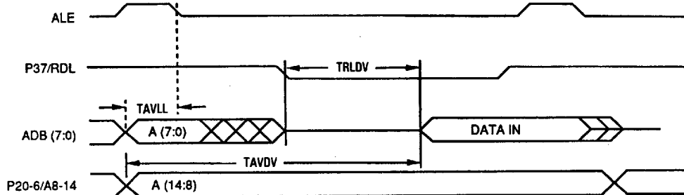
Figure 5. External Data Memory Read
