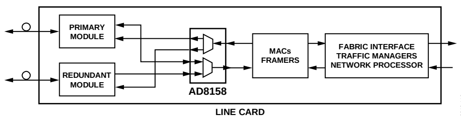
Figure 44. Using the AD8158 for Module Redundancy
