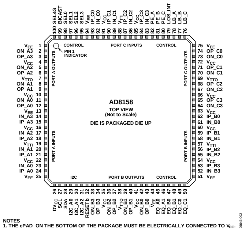
Figure 3. Pin Configuration
