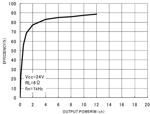
Fig.17 Output power—Efficiency (RL=6Ω)
