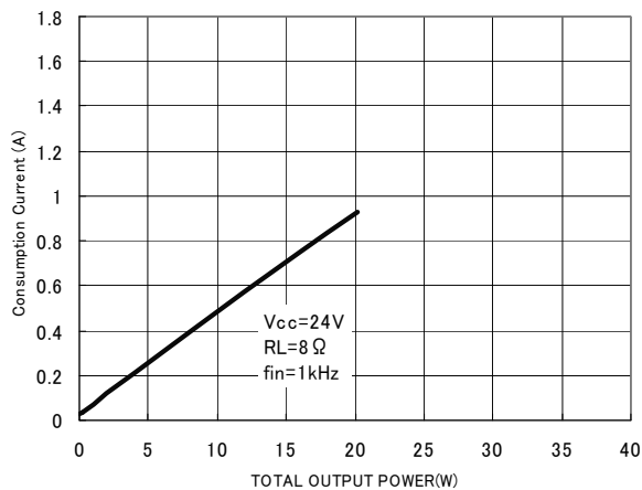
Fig.15 Total output power—Current consumption (RL=8Ω)
