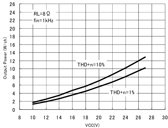
Fig.13 Power supply voltage—Output power (RL=8Ω)
